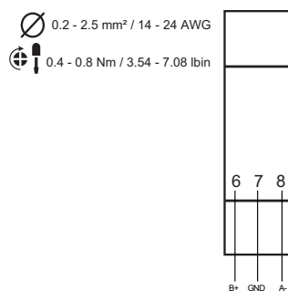
Fig. 8 Puerto RS485
