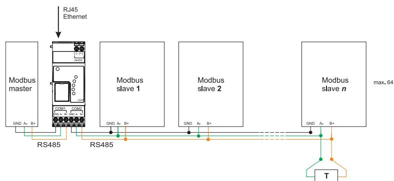
Fig. 2 Modbus RTU connection. COM 1 slave, COM 2 master
